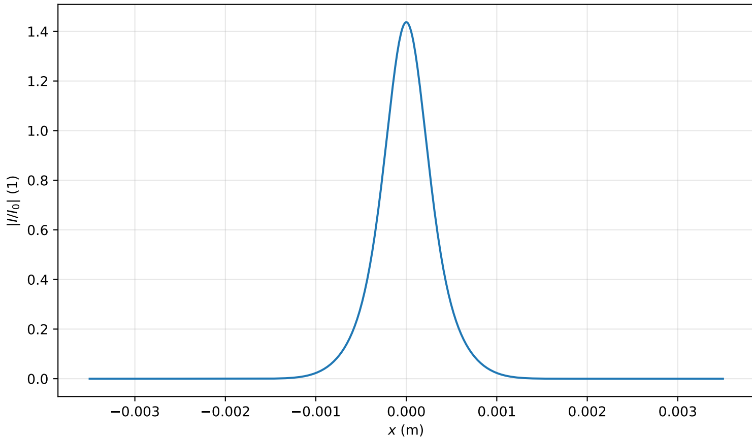
Intensity profile I(x, y = 0, z = 0.876m)/I_0 , P_{in}=1.0P_{cr} , artificial time
